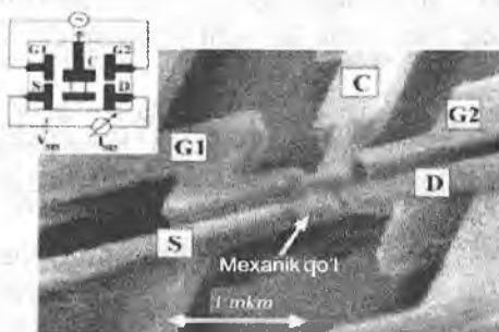
4.28-rasm. Blaykning nanomexanik ossilyatori.
