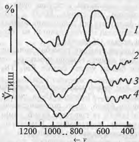
16-расм. Кристалларнинг ИҚ нур ютиш спектрлари: 1- \text{CaSiO}_3 ; 2- \text{La}_{9,34}(\text{SiO}_4)_6\text{O}_2 ; 3- \text{Ca}_{16}\text{La}_8\text{Al}_8\text{Si}_{16}\text{O}_{72} ; 4- \text{Ca}_{16}\text{Nd}_8\text{Al}_8\text{Si}_{16}\text{O}_{72} .
