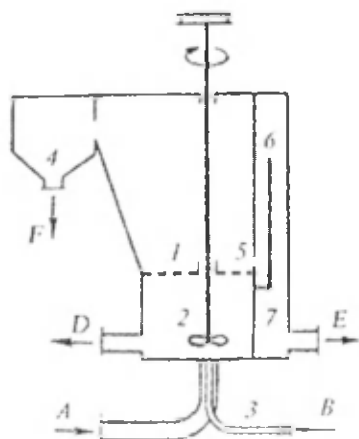
42-rasm. Aralashtirib flotatsiyalash mashinasining bo'limasi:
