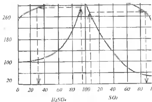
56-rasm. Atmosfera bosimida \text{H}_2\text{O}-\text{SO}_3 sistemasining qaynash diagrammasi.
