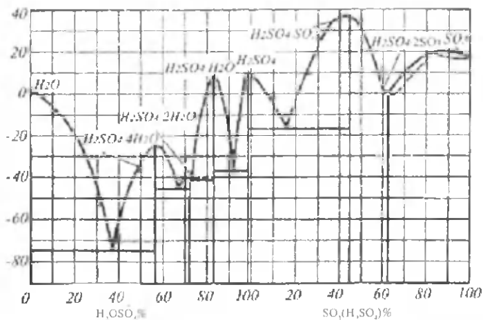
55-rasm. \text{H}_2\text{SO}_4 sistemaning kristallanish diagrammasi.
