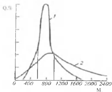
112-rasm. Polimerlarda molekularlarning molekular massasi bo'yicha taqsimlanishi: 1 — nitrotselluloza; 2 — polistirol.
