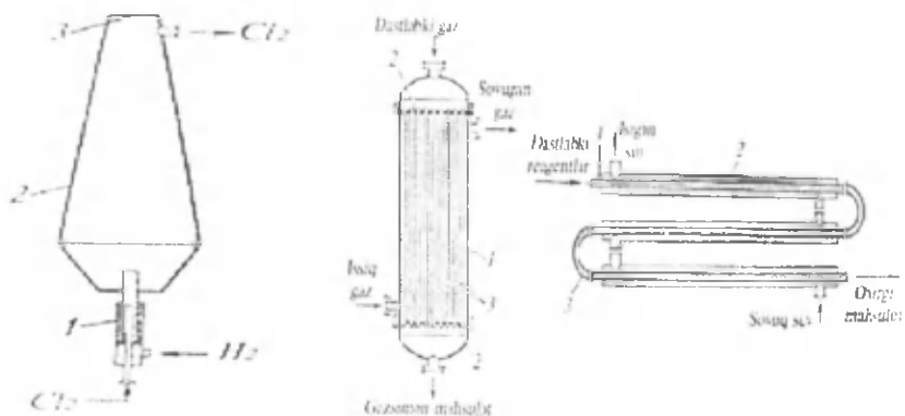
22- rasm. Vodorod-xlorid sintezlash pechi:
