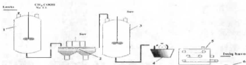
128-rasm. Lateksdan kauchuk olish sxemasi: 1 — koagulyator; 2 — tebranuvchi elak; 3 — yuvuvchi apparat; 4 — vakuumli baraban filtri; 5 — quritgich.
