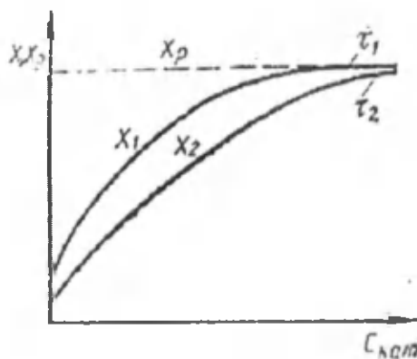
24-rasm. X moddaning \tau_1 va \tau_2 vaqtida \tau_2 > \tau_1 bo'lganda ( \tau va p = \text{const} ) mahsulotga aylanish darajasiga katalizator konsentratsiyasining ta'siri.
