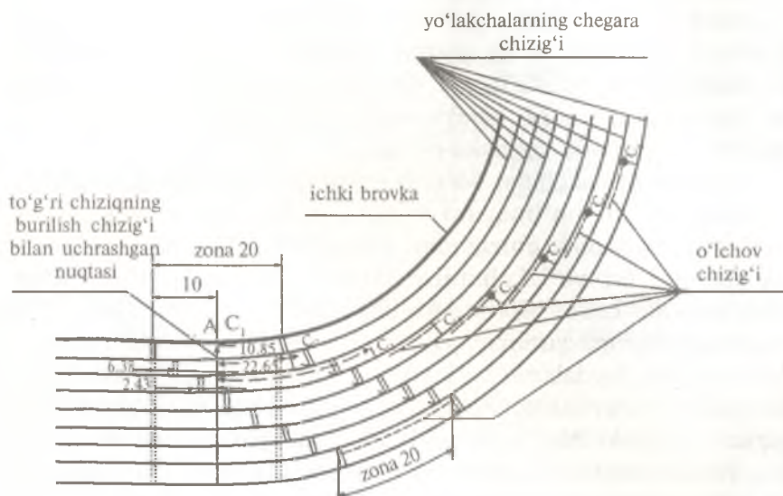
21-rasm. 4×200 va 4×400 m ga estafetali yugurishda alohida yo‘laklardan yugurish uchun birinchi uch burilish.
