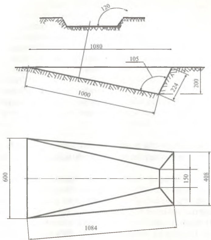
10-rasm. Langarcho'p bilan tayanadigan quti (mm).
