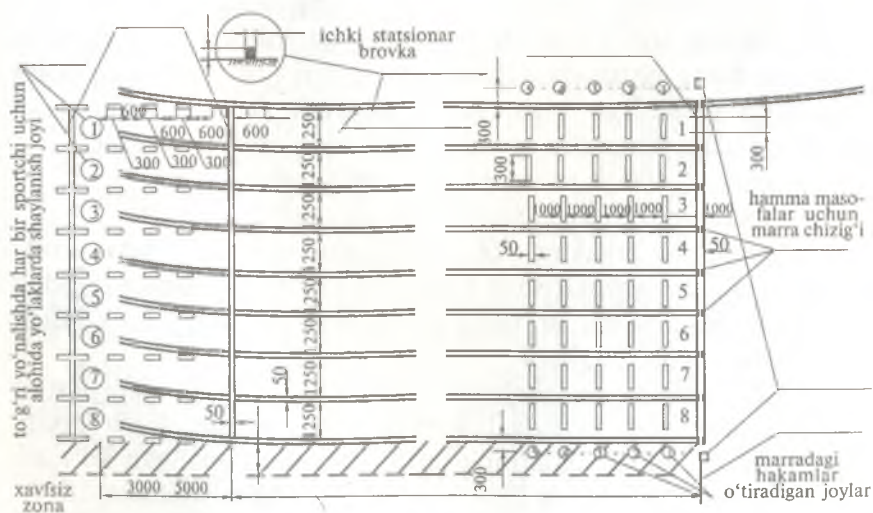
2-rasm. 100 m li masofaga yugurishda shaylanish va marra chiziqlari, mm.
