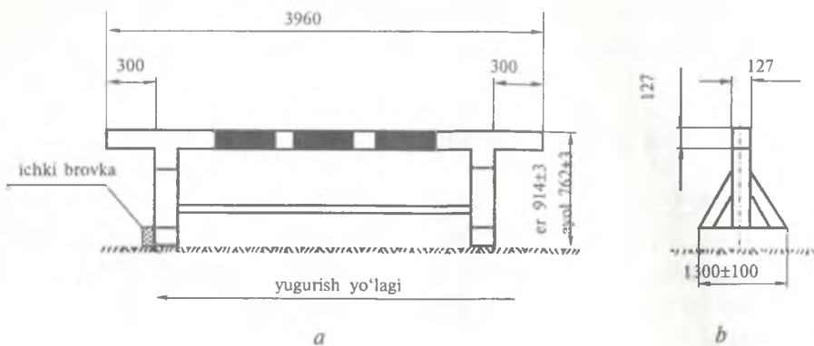
4-rasm. Stipel-chez to'siqlari, mm: a —olddan ko'rinish, b —yondan ko'rinish.
