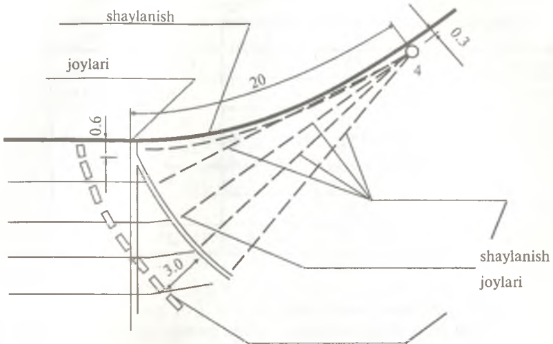
18-rasm. Buriishda shaylanish joyini belgilash.
