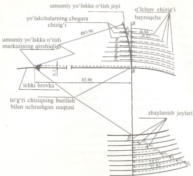
20-rasm. 800 m ga yugurishda alohida yo'lakchalardan yugurish uchun shaylanish chizig'ini belgilash (birinchi burilishda).
