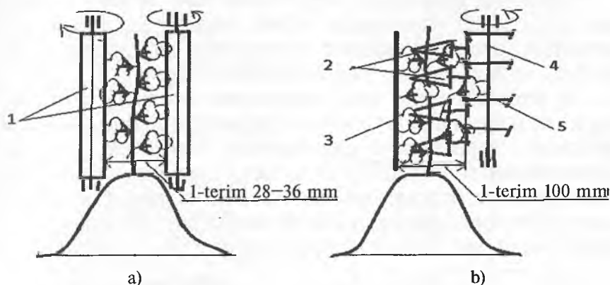
2.29-rasm. Paxtani tik (a) va gorizontall (b) shpindelli terish apparati bilan terib olish jarayonlari:
