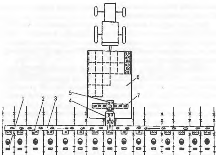
2.45-rasm. AUS-0,1 sabzavotlarni qo'lda terib olish agregati: 1 – o'tirish joyi; 2 – yashik-yig'gich; 3 – ko'ndalang transporter; 4 – ko'tarish transporteri; 5 – yashik; 6 – platforma; 7 – yashik-ta'minlagich.
