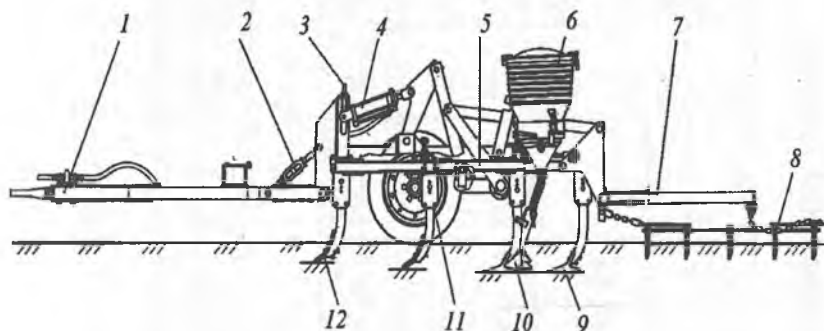
2.11-rasm. ChKU-4A chizel-kultivatorining tuzilishi: 1 – tirkagich; 2 – roslash vinti; 3 – tortuvchi vint; 4 – gidrosilindr; 5 – rama; 6 – o'g'it sepish apparati; 7 – molalar uchun rama; 8 – sixli mola; 9 – o'q-yoysimon panja; 10 – ekkich; 11 – g'ildirak; 12 – yumshatuvchi panja.
