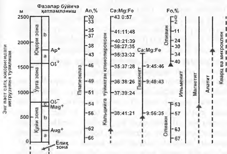
1.7-rasm. Skayergaard intruziyasidagi kumulat minerallarining o'zgaruvchanligi. Qisqartmalar: Mg - magnetit; Aug - piroksen; Ol - olivin; Ap - apatit; An - anortit; Fo - forsterit (Ch.Xyudjes, 1988)
