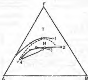
4.4-rasm. AFM diagrammasida har xil kimyoviy seriyalar o'rni (Jrwin, Baragar, 1971).
