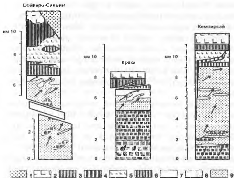
4.16-rasm. Uralofiolitlarining soddalashtirilgan kesmalari (A.A.Knipper, G.N.Savelyeva, A.Ya.Sharaskin bo'yicha).
