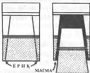
1.2-rasm. Atrof jinslarining cho'kishi natijasida magmatik o'choqlar hosil bo'lish sxemasi (Ramberg, 1977)
