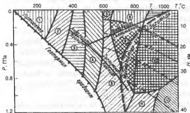
2.7-rasm. Metamorflashgan gilli jinslarning mineral fatsiyalari (A.A. Marakushev, 1988).
