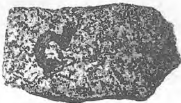
4.95-rasm. Sienit.
