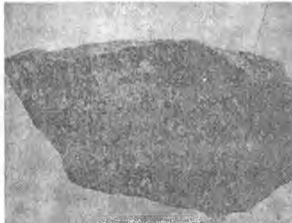
4.34-rasm. Normal granit.
