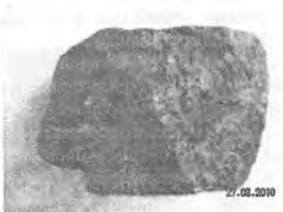
6.20-rasm. Gneys.
