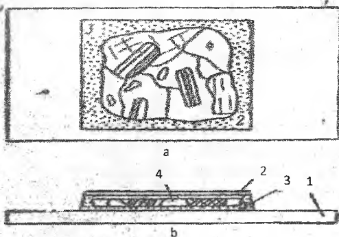
1.9-rasm. Petrografik shlif:
