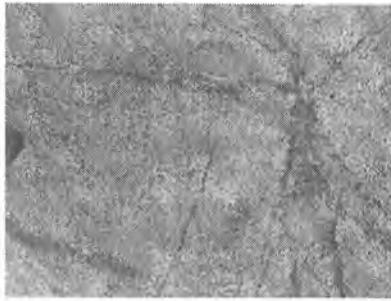
4.93-rasm. Gornblendit. Nikollar +
