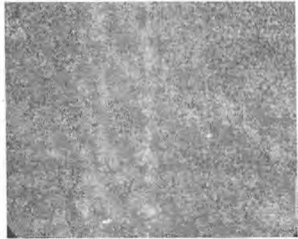
6.10-rasm. Gilli slanes. Nik.+
