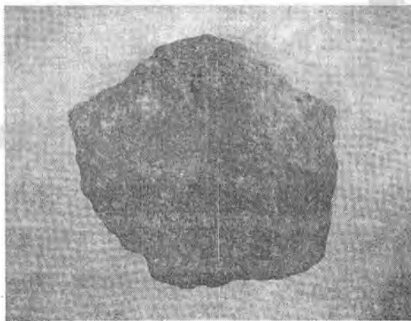
4.38-rasm. Porfirimon granit.
