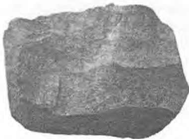
5.32- rasm. Liparit-tufi.
