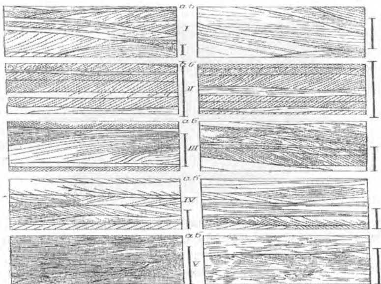
5.14 - rasm. Har xil genezisli hozirgi (a) va qadimgi (b) yotqizilardagi qiya qatlamlanishga misollar ( A.V.Xabakov, 1952). Qiya qatlamlanish: I – shamolli; II – davriy oqimlarniki; III – yirik daryolarniki (a- d. Volga); IV – deltaniki; V – dengiz qirg‘oq oldiniki. Rasmlarda chizg‘ich masshtabi 1 metrga teng.
