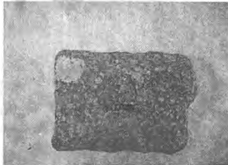
4.102-rasm. Traxit.
