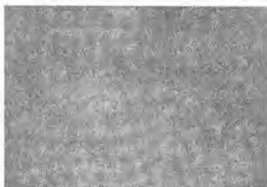
4.57-rasm. Obsidian. Nikollar +
