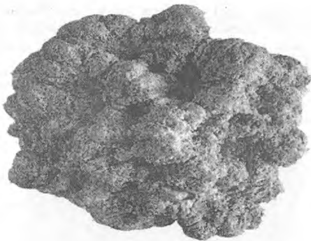
5.40-rasm. Kremniy tufi.
