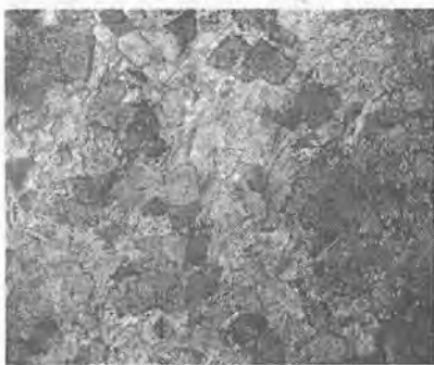
5.55-rasm. O‘rta donali dolomit. Nikollar +
