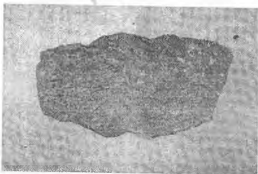
4.54-rasm. Felzit.
