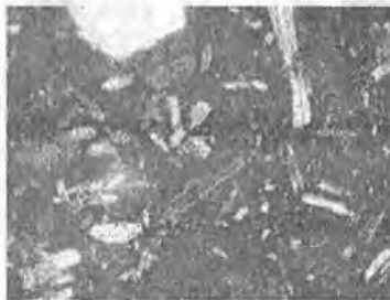
4.94-rasm. Pikrit-porfirit. Nikollar +
