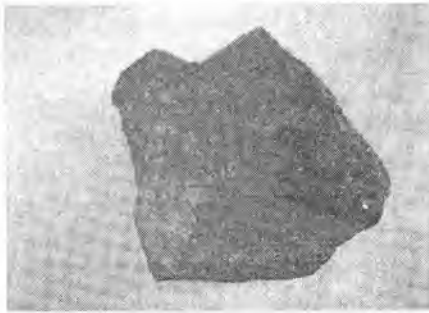
4.43-rasm. Mikrogranit.
