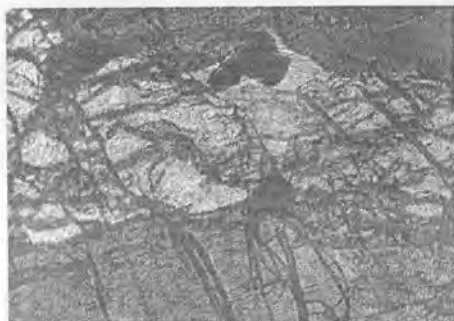
4.88-rasm. Dunit. Nikollar +
