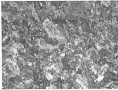
4.63-rasm. Kersantit. Nikollar +
