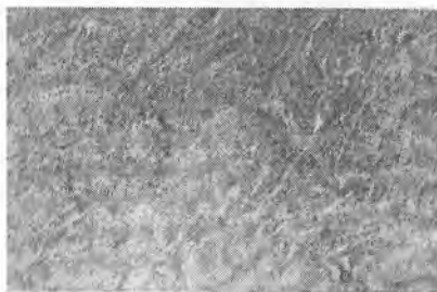
4.56-rasm. Felzit. Nikollar =
