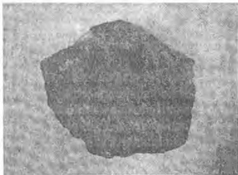
4.32-rasm. Porfirsimon granit.
