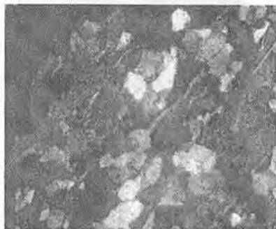
6.18-rasm. Kvars-biotitli slanes. Nik.+
