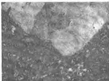
4.103-rasm. Ortofir.
