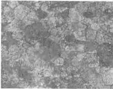
6.27-rasm. Kalsit tarkribli marmor. Nikl +Dolomit. Nikl +
