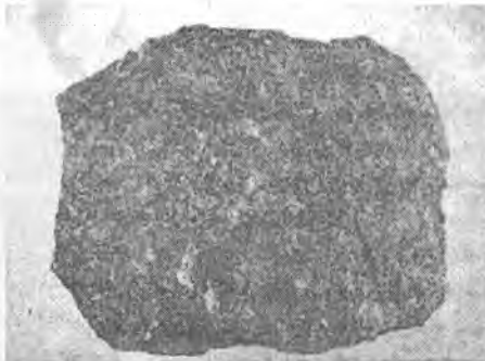
4.73-rasm. Labrodorit.
