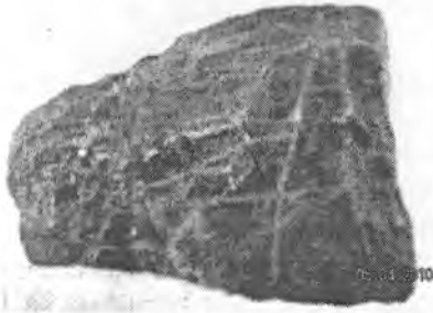
6.9-rasm. Gilli slanes.
