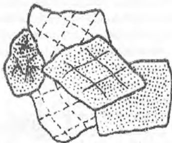
2.5-rasm. Shlifdagi minerallarning turlicha g‘adir-budurligi.
