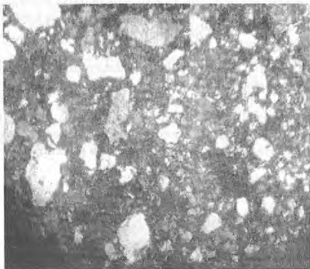
5.21-rasm. O'rta donali psammit strukturali qumtosh. Nikollar +
