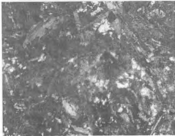
4.77-rasm. Diabaz. Nikollar +
