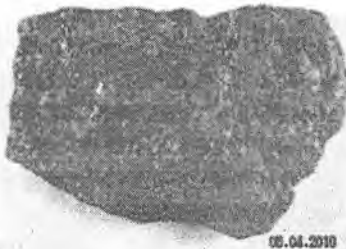
6.11-rasm. Amfibol xloritli slanes.
