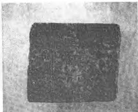
4.68-rasm. Gabbro teng donali.
