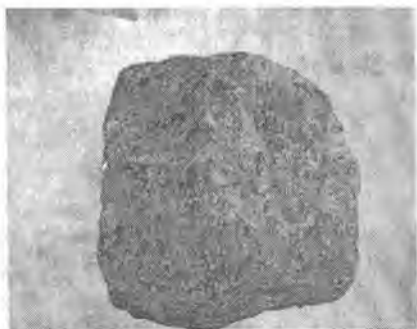
4.36-rasm. Alyaskit.
