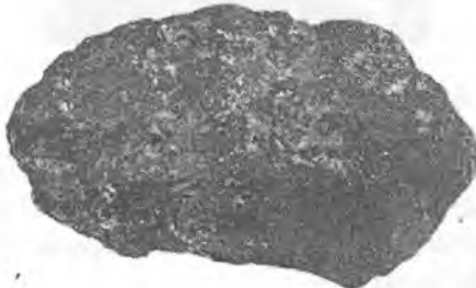
4.92-rasm. Gornblendit.
