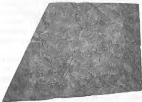
5.18- rasm. Tektonik brekchiya.
