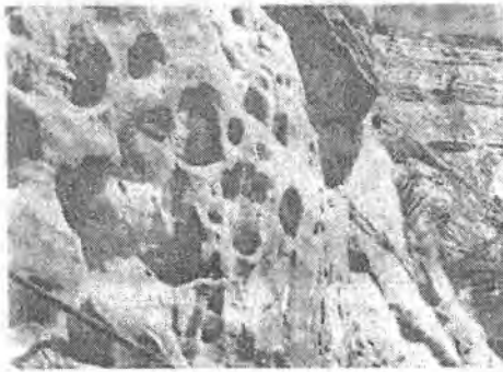
5.1 - rasm. Quyi bo‘r qumtoshining shamol ta‘sirida tuxumsimon nurashi.
