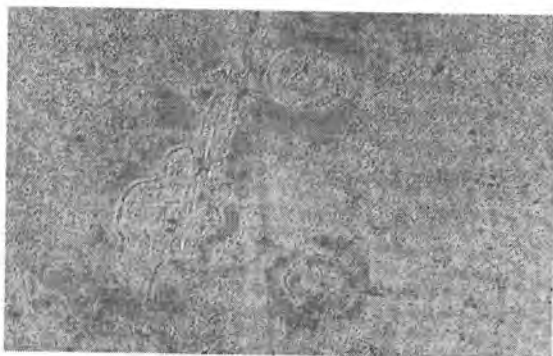
4.53-rasm. Obsidian. Nikollar =
