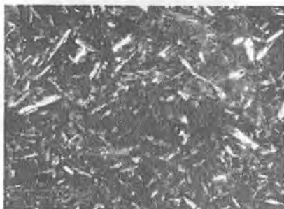
4.84-rasm. Bazalt. Nikollar +
