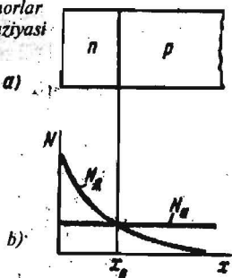
III.57-rasm. Diffuzion p-n o'tishning hosil bo'lishi.
