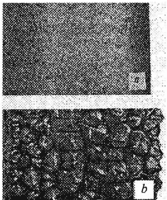
II.26 – rasm. Vodorod bilan tiklash jarayonida olingan sterjenlar sirtining ko'rishi: a – optimalga yaqin; b – undan uzoq.
