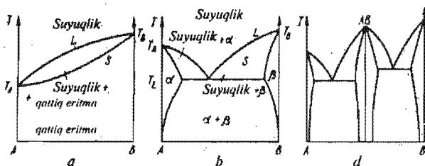
II.1 — rasm. Fazalar diagrammalarining eng muhim hollari:
