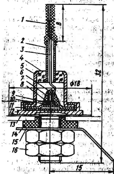
III.63-rasm. Kremniy yassi diodning tuzilishi chizmasi:
