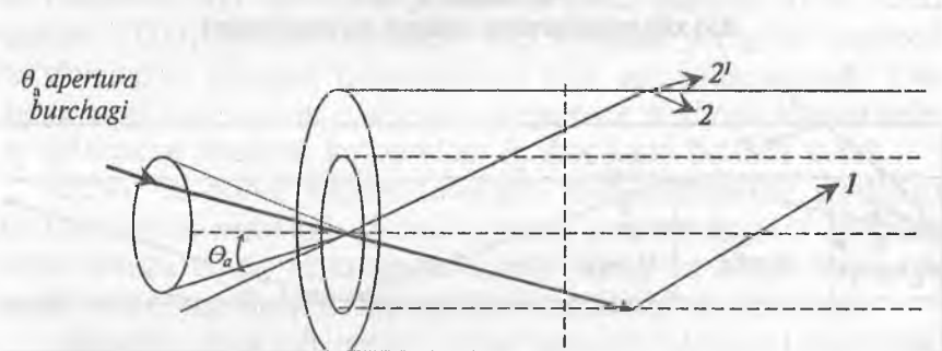
2.13-rasm. Optik tolaning apertura burchagi
