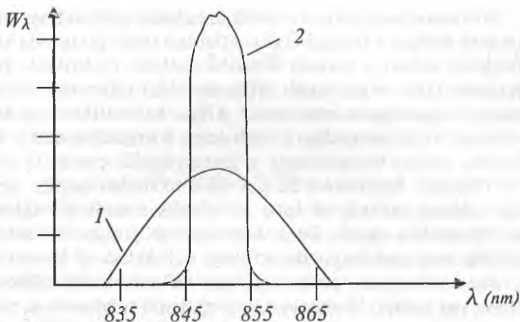
3.15-rasm. Gallyiy arsenidili injeksion lazerning spektral xarakteristikasi
