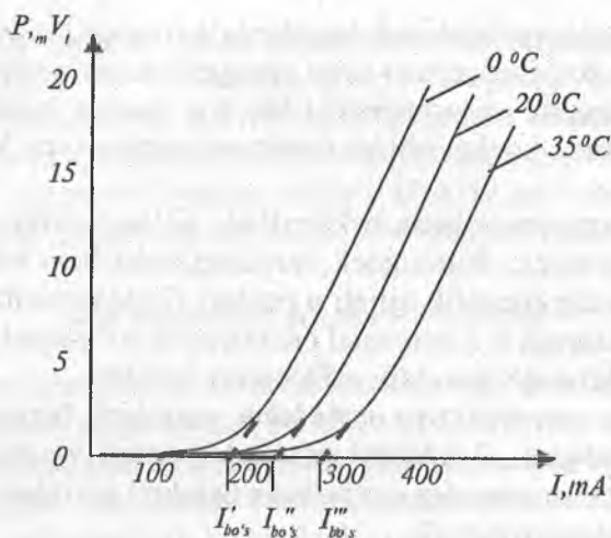
3.19-rasm. Lazer diodi vatt-amper xarakteristikasining haroratga bog'liq ravishda o'zgarishi
