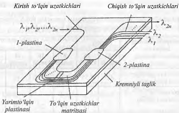
9.5-rasm. Tolali optik multipleksorning tuzilishi
