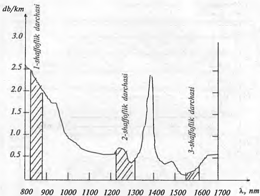
2.7-rasm. To'liq uzunligiga bog'liq ravishda optik toladagi so'nishning o'zgarishi
