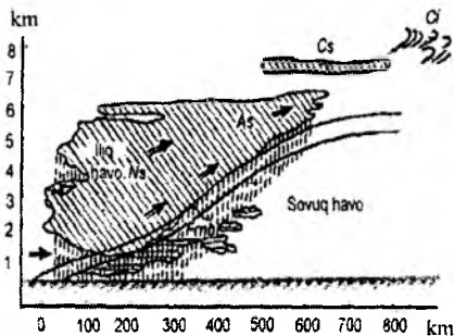
10.3-rasm. Iliq front chizmasi
