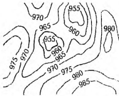
2.1-rasm. Izobaralar
