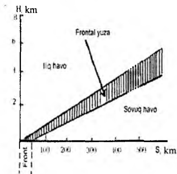
10.2-rasm. Frontal yuza va front chizmasi
