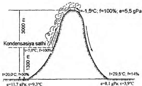
9.5 - rasm. Fyon shamolining hosil bo'lishi
