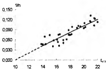
14.1-rasm. Chigit unib chiqish tezligining o'rtacha sutkalik havo haroratiga bog'liqligi
