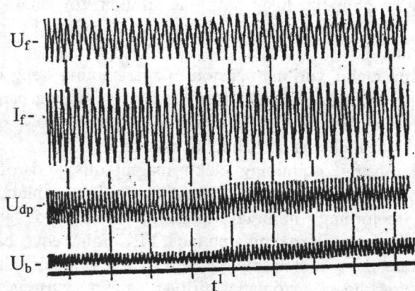
5.2-rasm. Boshqaruv signali musbat qiymatli chastotasi rostlanadigan elektr yuritmaning energiya tejamlor ish rejimlari ossillogrammalari
