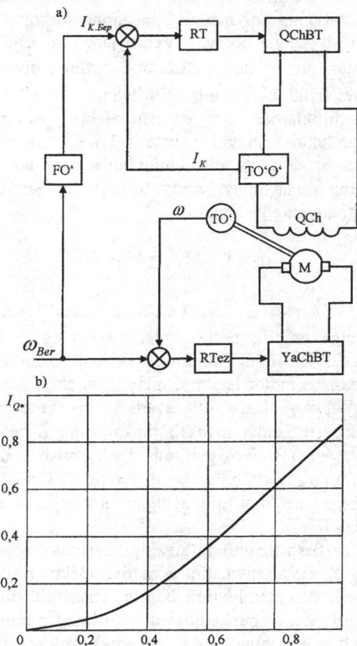
3.3-rasm. Ventilatorli yuklanishli mexanizmning o'zgarmas tok elektr yuritmasi:
