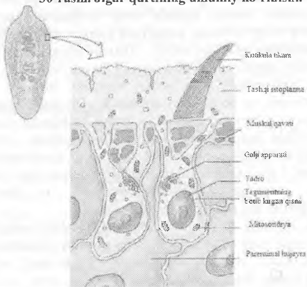
31-rasm 20 . Jigar qurti ( Fasciola hepatica ) teri qatlami tuzilishining ko'rinishi.
