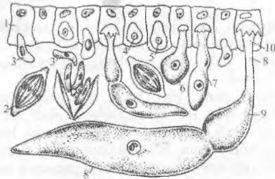
10-rasm. Gregarinalarning rivojlanishi:
