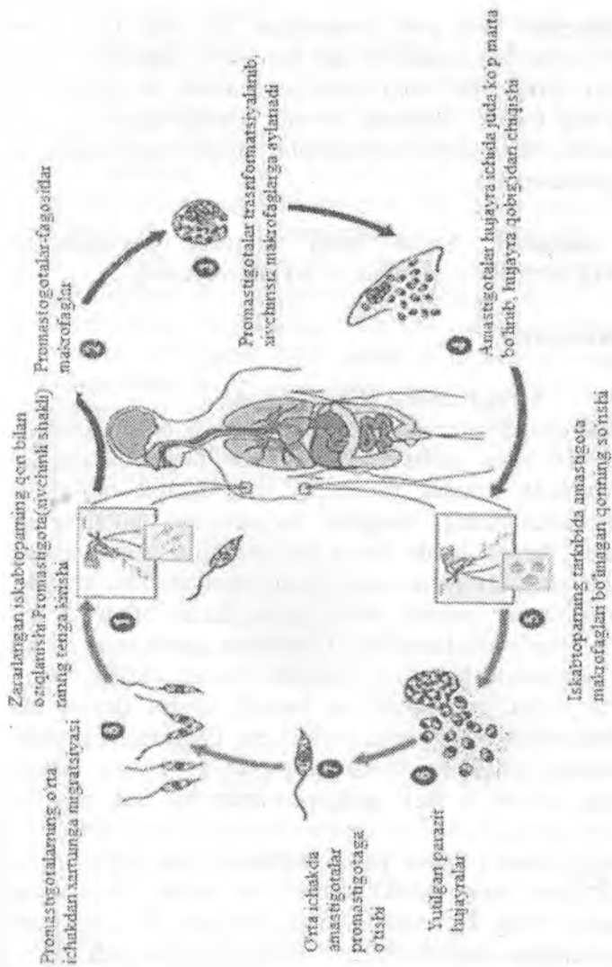
8-rasm 5 . Leishmaniyaning rivojlanish sikli.
