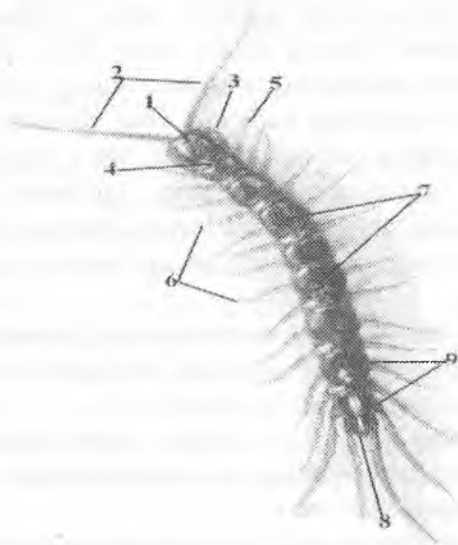
61-rasm. Kostyanka – Lithobius forticatus ning tuzilishi.
