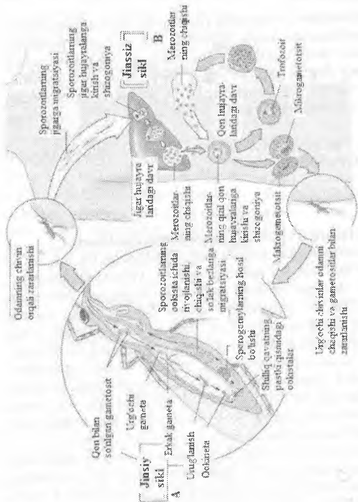
11-rasm 6 . Bezgak plazmodiysining rivojlanish sikli.
