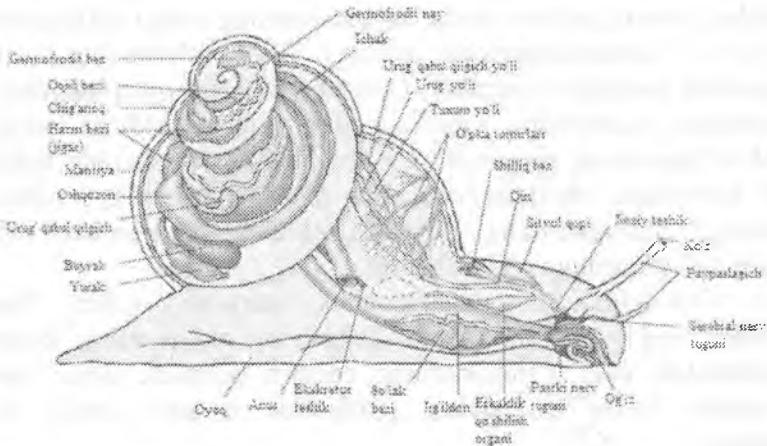
42 rasm 28 . Tok shilliqurtining ichki tuzilishi.
