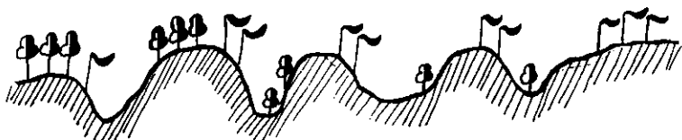
4-rasm. V. V. Alyoxinning o'simliklarning taqsimlanish sxemasi
