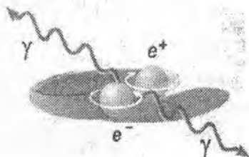
4.3-rasm. Gamma-kvant hosil bo'lishi
