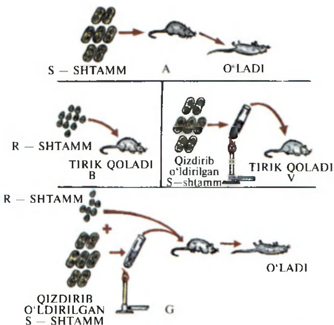
70-rasm. Griffit tajribasining sxemali ifodasi:
