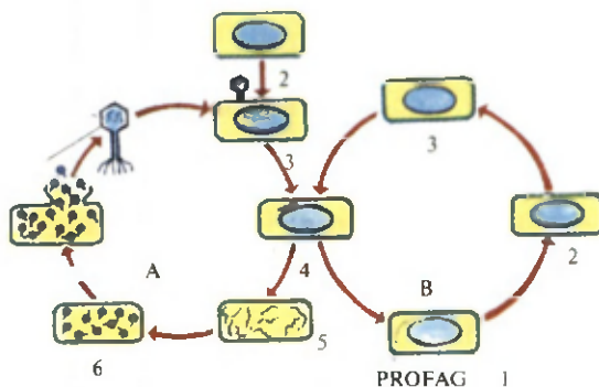
72-rasm. Faglarning hayot sikli:
