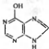
gipsoksanthin
