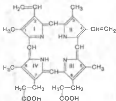
Protoporfirin-IX
