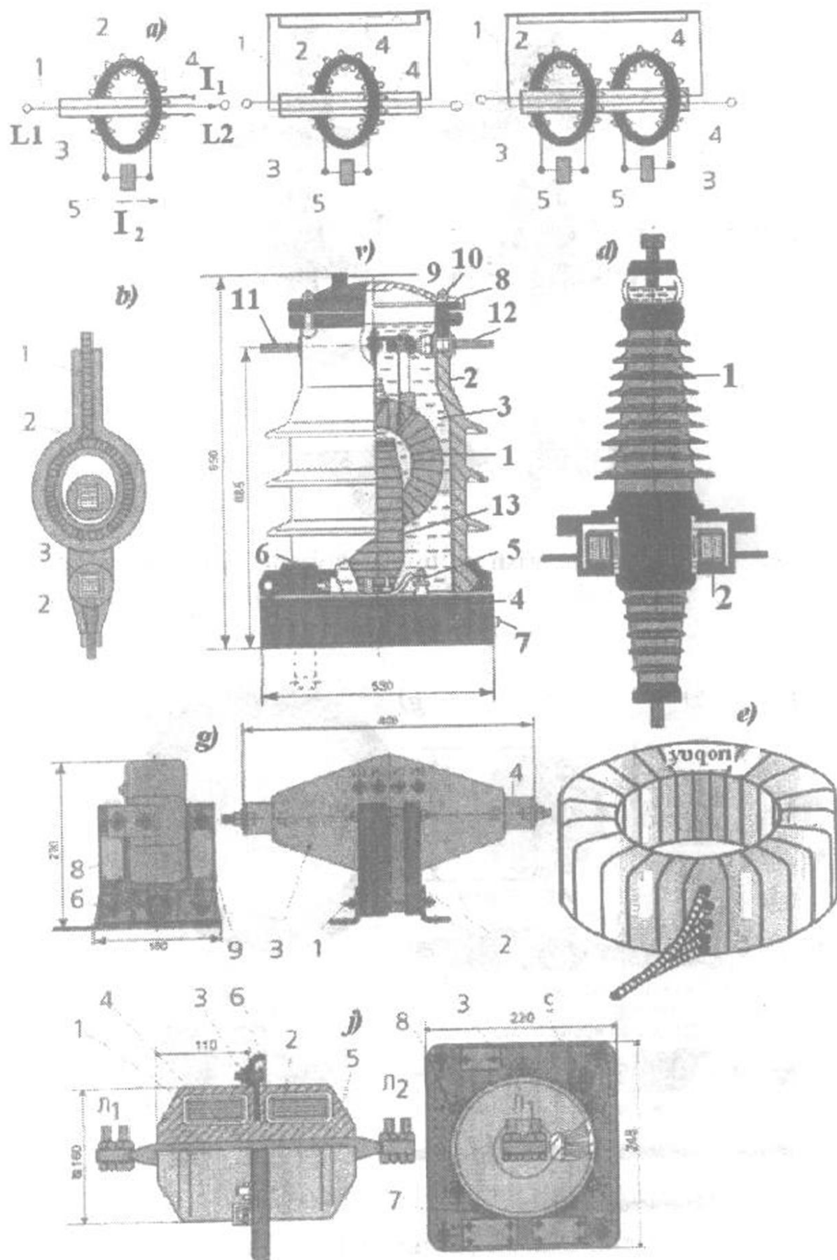
35-rasm. Tok transformatorlari
