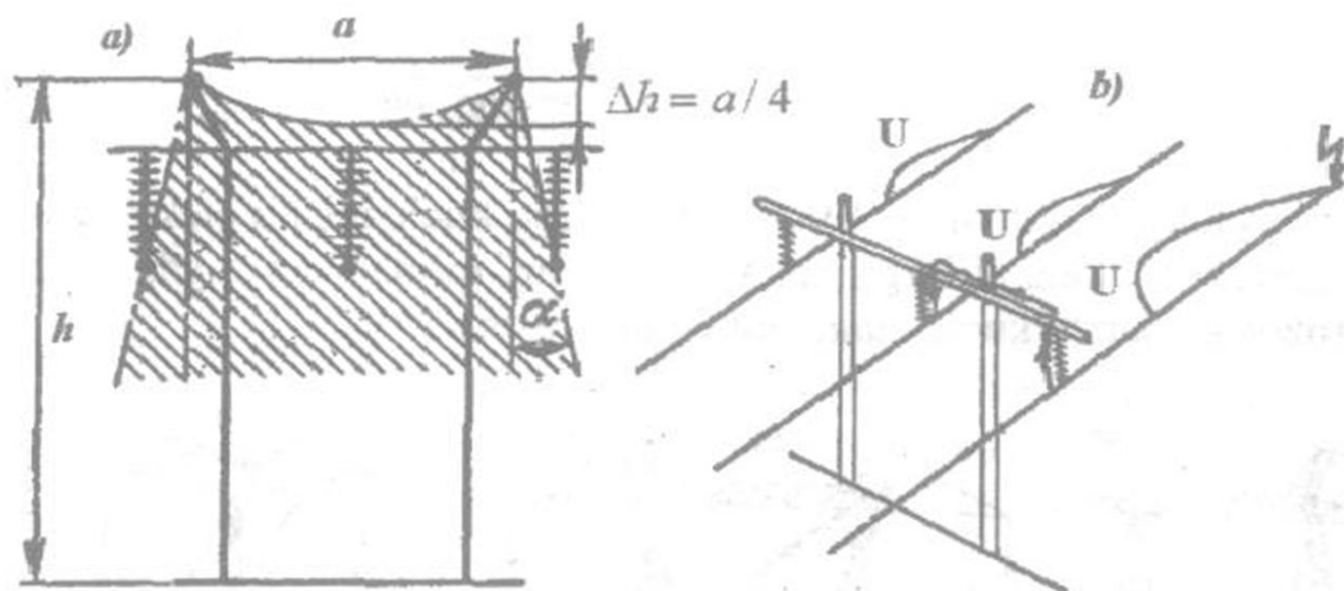
50-rasm. Havo elektr uzatish yo'llarini yashindan himoyalash
