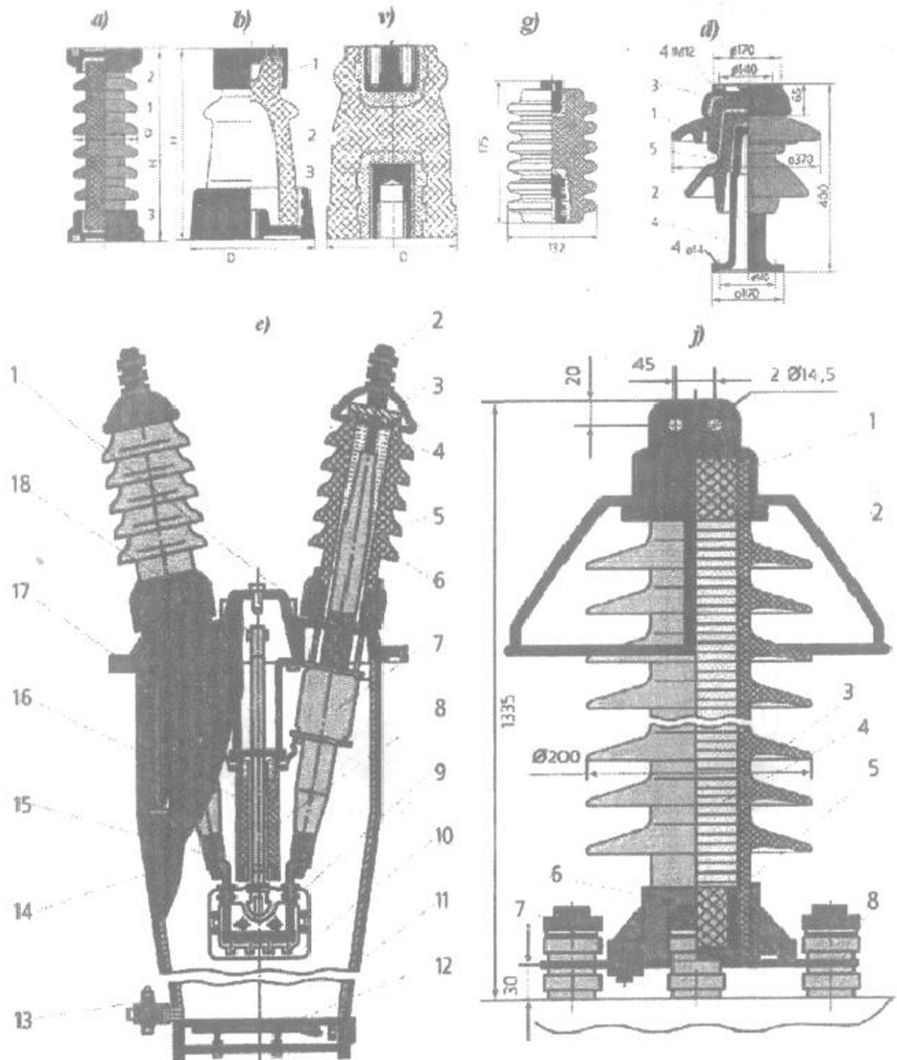
9-rasm. Tashqi tayanch (a) va stansion (b,v,g) izolyatorlar, 35 kV nayzabop ikki likobchali izolyator (d), 35 kV o'chigich C-35 kirma izolyatori (e), 3 kV dan 110 kV gacha yarim o'tkazgichli o'takuchlanishni chegaralagich (j).
