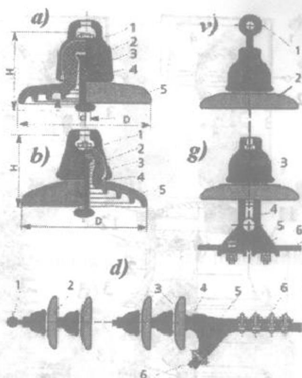
24-rasm. Havo elektr uzatish yo'lining likobcha izolyatorlari (a, b), likobcha izolyatorni osish usullari (v, g), tortna likobcha izolyatorlar girlyandasi (d).
