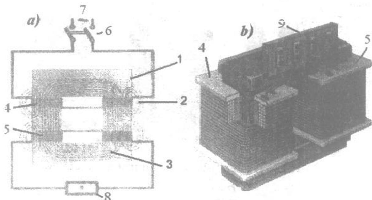
61-rasm. Transformatorning ishlash prinsipi (a) va tuzulishi (b).
