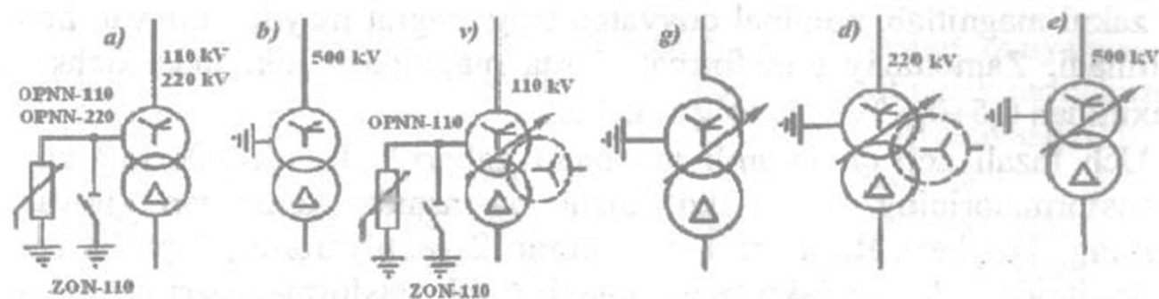
63-rasm. Transformator neytralini yerlash
