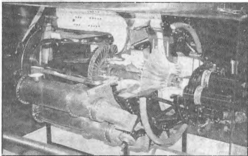
5.3-rasm. Radial markazdan qochma kompressor bilan prepartlangan TRD General Electric J-31.
