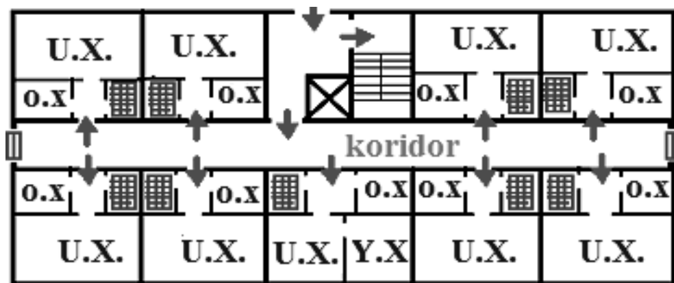
4.19-rasm. Koridorli turar-joy binosining loyihaviy yechimi
