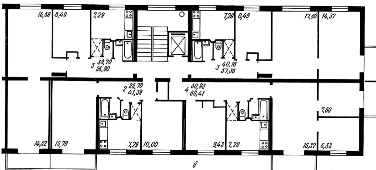
4.14-rasm. 9-qavatli bo'linmali turar-joy binosining o'ng tomondagi T-2-3-3-4 blok bo'linmasi
