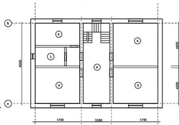
4.4-rasm. Ikki qavatli individual turdagi turar-joy binolarining tarzlari va tarhlari
