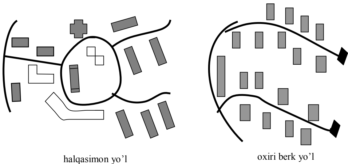
6.6-rasm. Mikrorayon bo'ylab transport harakatlanish yo'llari
