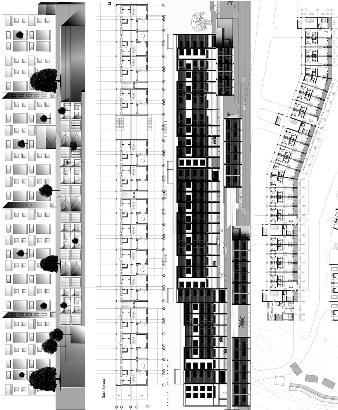
4.18-rasm. Yo'lakli turar-joy binolarining tarzi va tarhiga oid namunalar
