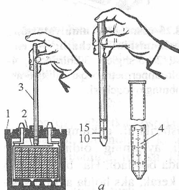
18.23-rasm. Akkumulyatoridagi elektrolitning sathini tekshirish: a -shisha naychali o'lichagich orqali; b -chamalash orqali; 1-korpus; 2-himoya chambaragi; 3-naycha; 4-naychanning shkalasi; 5-quyish teshigi.
