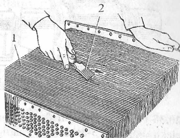
20.37-rasm. Radiator plastinkalarini to'g'irlash: 1-radiator; 2-to'g'irlagich.
