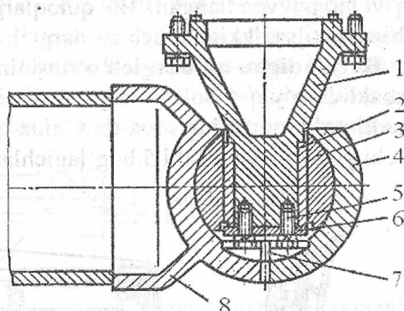
6.4-rasm. Brusning sharli tayanchi: 1-traktor ramasidagi tayanch o'q; 2-vtulka; 3-segmentsimon vtulka; 4-sharsimon qopqoq; 5-bolt; 6-shayba; 7-to'g'rilagich; 8-balkaning sharsimon tayanchi.
