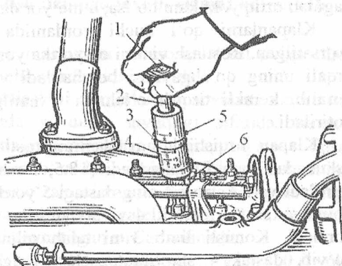
18.4-rasm. KH-723 rusumli asbob: 1-dastak; 2-shtok; 3-prujinali halqa; 4-korpus; 5-vint; 6-asbobning oyog'i.
