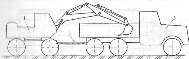
3.3-rasm. Shatakka olib transport qilish: 1-ekskavator; 2-shatak; 3-tortuchi avtomobil.
