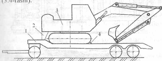
3.4-rasm. Ekskavatorni trayler yordamida transport qilish: 1-trayler; 2,4-tirkaklar; 3-ekskavator.
