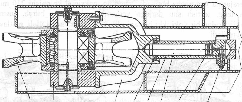
18.20-rasm. Zanjirli tasmani gidravlik usulda tortish: 1-yetakchi g'ildirak; 2-sirpangich; 3-ayriq; 4,7-moy tutkichlar; 5-silindr; 6-plunjer; 8-klapanli moydon.
