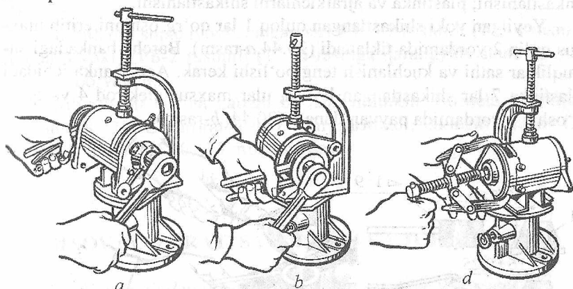
20.42-rasm. Generator detallarini bo'laklarga ajratish: a -yakor gaykasini burash; b -shkiv gaykasini burash; d -yakorni maxsus moslama yordamida sug'irib olish.
