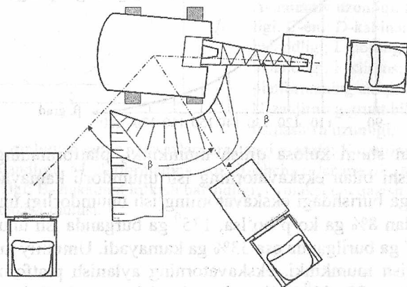
4.5-rasm. Yuklash jarayonini planda ko'rinish chizmasi.
