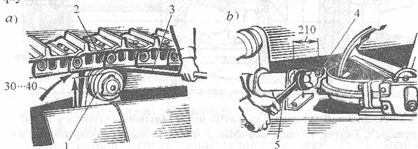
18.18-rasm. Tasmali zanjirni tekshirish va rostlash: a-zanjirni tekshirish; b-zanjirni rostlash; 1-rolik; 2-zanjirli tasma; 3-lom; 4-gayka; 5-kalit.
