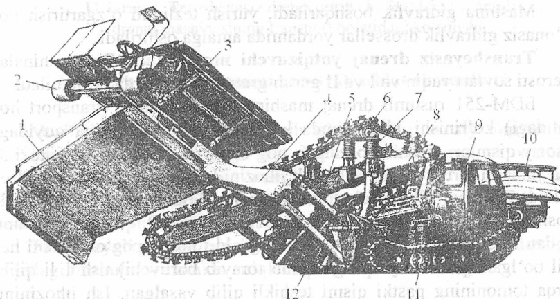
11.1-rasm. Transheyasi toraytirilgan DY-251 rusumli drenaj mashinasining transport holatidagi ko'rinishi.
