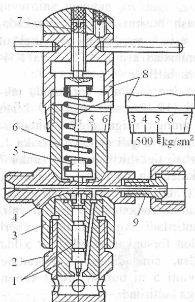
18.13-rasm. Maksimetrning qirgimi: 1-ignali changitgich; 2-gayka; 3-korpus; 4,9-shtutserlar; 5-shtift; 6-prujina; 7-rostlovchi bolt; 8-rostlovchi qalpoq.
