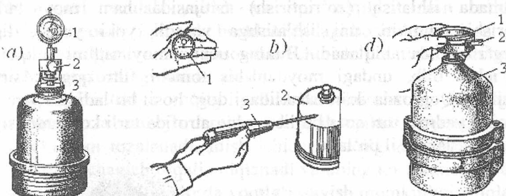
18.8-rasm. Rotorli sentrifuga: a -ifloslanish darajasini tekshirish; 1-soatli indikator; 2-rotorning indikator; 3-rotor qalpog'i; b -rotorni aylanish vaqtini o'lchash; 1-sekundomer; 2-rotor qalpog'i; 3-avtostetoskop; d -rotorning aylanish chastotasini o'lchash; 1-asbob; 2-tilcha; 3-rotor qalpog'i.
