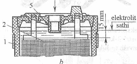
18.23-rasm. Akkumulyatoridagi elektrolitning sathini tekshirish: a -shisha naychali o'lichagich orqali; b -chamalash orqali; 1-korpus; 2-himoya chambaragi; 3-naycha; 4-naychanning shkalasi; 5-quyish teshigi.
