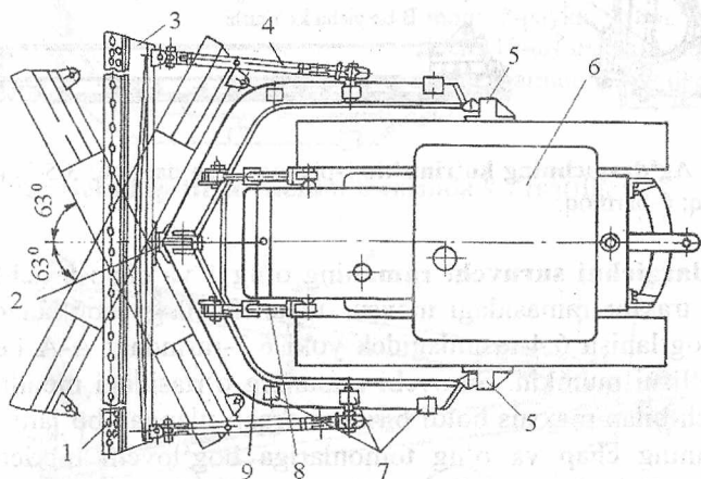
6.5-rasm. Ag'dargichi buraladigan buldozerning planda ko'rinishi.
