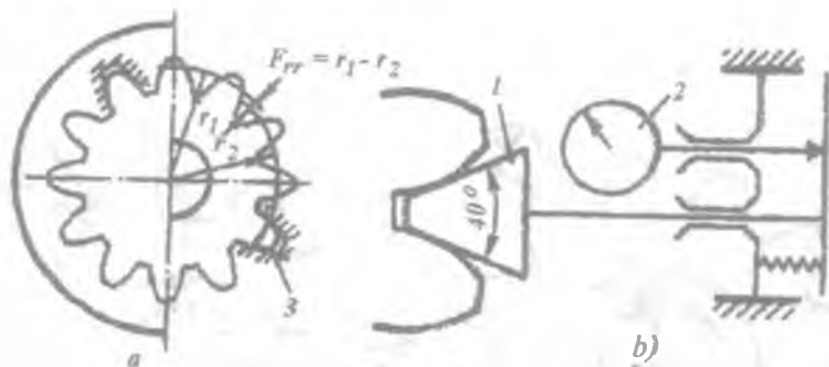
41-rasm. Tish gardishining radial tepishi (a) va tepishni o'ldash sxemasi (b).
