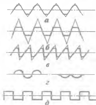
33-rasm. Rezbalarning profillari.
