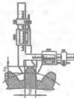
50-rasm. Shtangentish o'lchagich.
