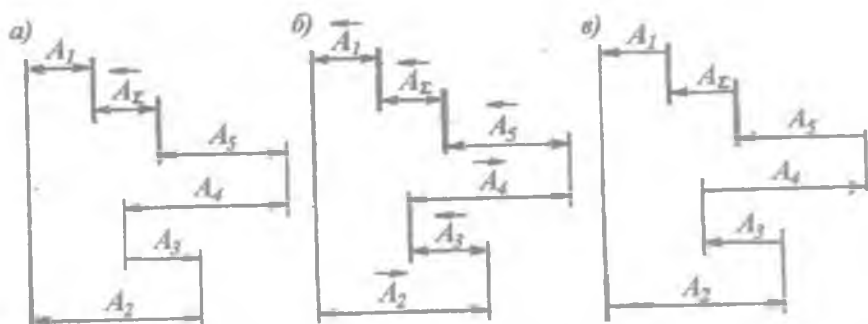
54-rasm. O'lchamlar zanjirlari zvenolarini tartiblash.
