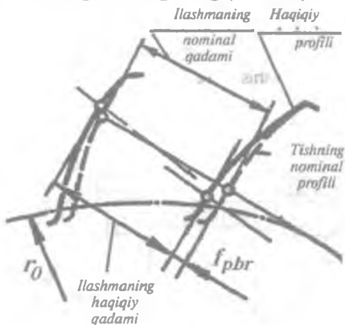
44-rasm. Tutashish qadamining og'ishi.
