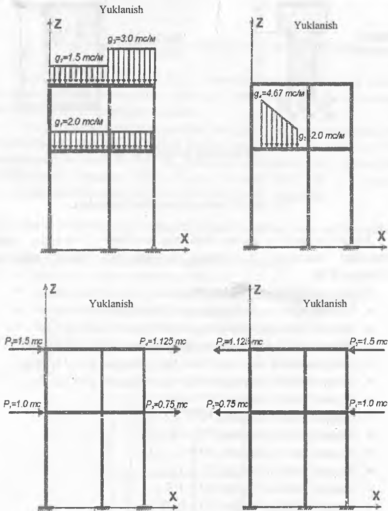
5.3-rasm. Ramaning yuklanish sxemasi.
