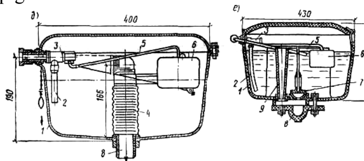
3.1- rasm. Qavatlangan sifon bilan jihozlangan yuvish bachogi
