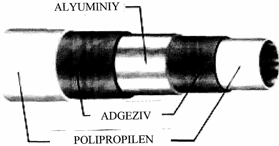
1.2. rasm. Metalpolipropilen quvurlar
