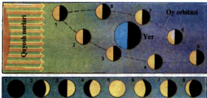
33- rasm. Oy fazalarining almashinishi
