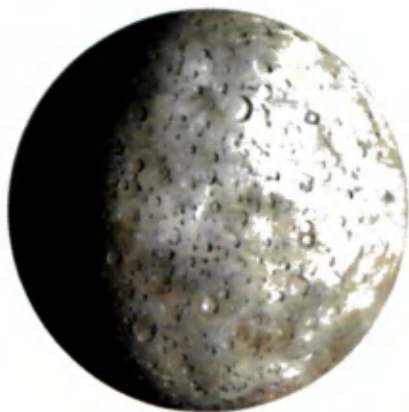
71- rasm. Merkuriy sirti («Mariner-10» KA olgan rasm).
