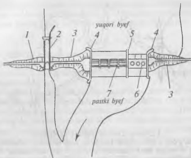
3.12-rasm. GESli suv inshooti majmuasining chizmasi.
