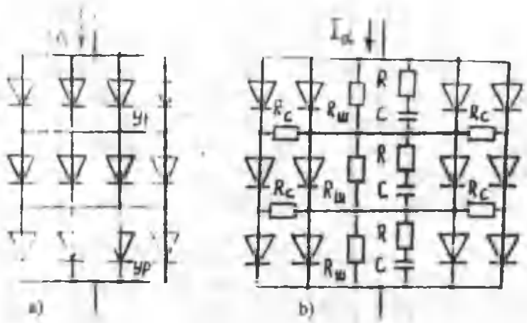
9.18-rasm. Ventillarni ketma-ket parallel ulash sxemasi.
