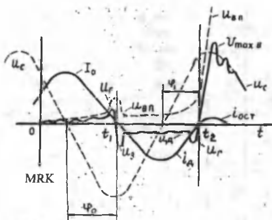
4.5-rasm. Past kuchlanishli zanjirning uzilishidagi jarayon.
