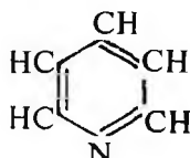
piridin
