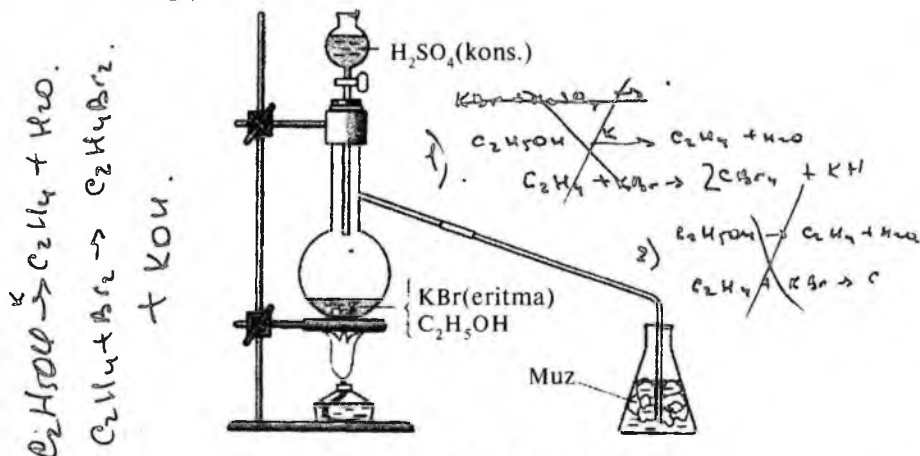
7-rasm. Etanoldan brometan olish.
