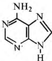
adenin (a)
