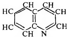
xinolin
