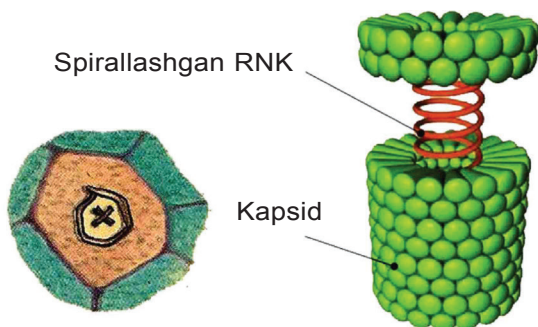
Virusning tuzilishi
