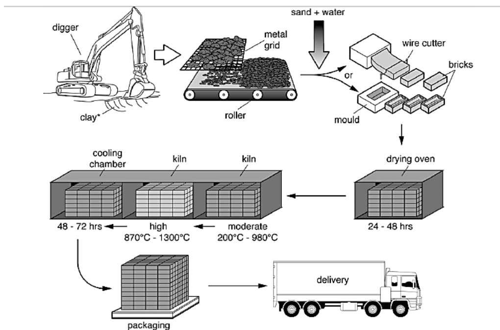
Brick Manufacturing
