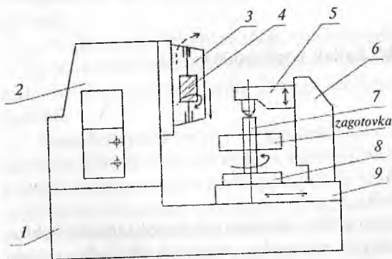
14.1-rasm. Tish frezalash stanogi.
