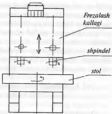
12.5-rasm. 621 modelli karusel-frezalash stanogi.
