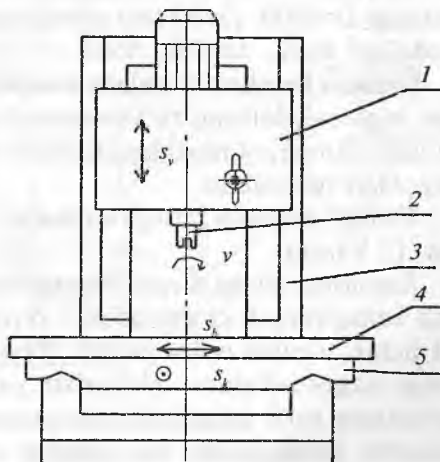
12.2-rasm. Krest stolli konsolsiz vertikal frezalash stanogi: 1-shpindel babkasi; 2-shpindel; 3-stanina; 4-stol; 5-karetk.
