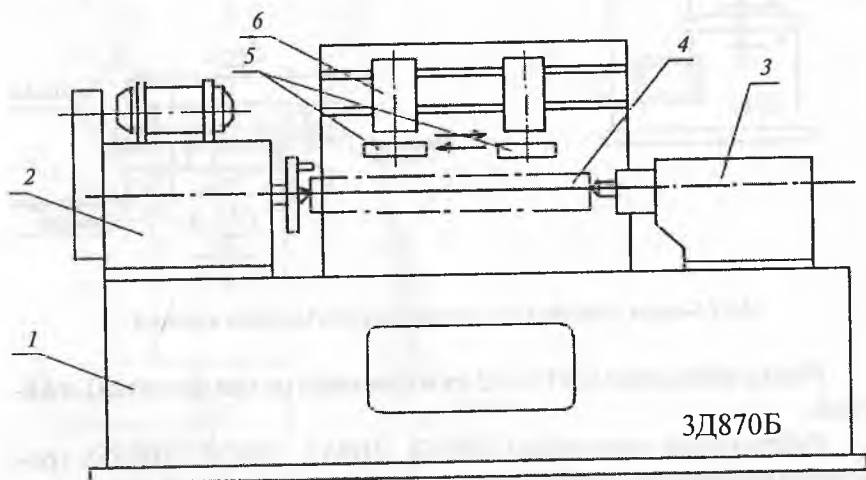
16.16-rasm. Superfinishlash stanogi:
