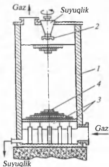
29- rasm. Nasadkali minora.
