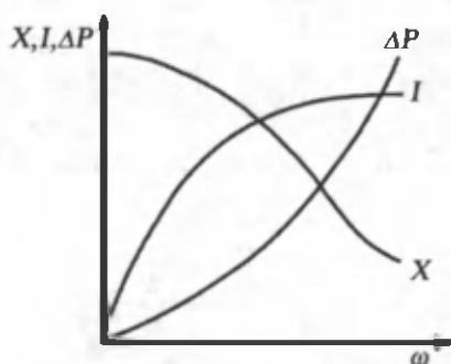
23- rasm. Apparatda gaz tezligi \omega ortganda mahsulotga aylanish darajasining ish intensivligining I va gidravlik qarshilikning \Delta P o'zgarishi.
