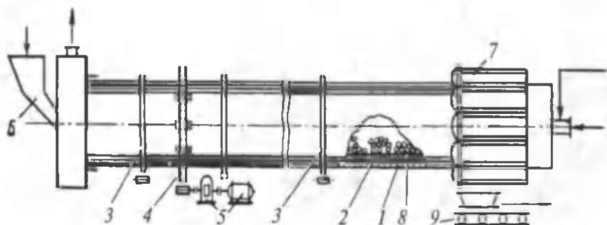
39- rasm. Sement klinteri ishlab chiqarish uchun aylanuvchi barabanli pech.
