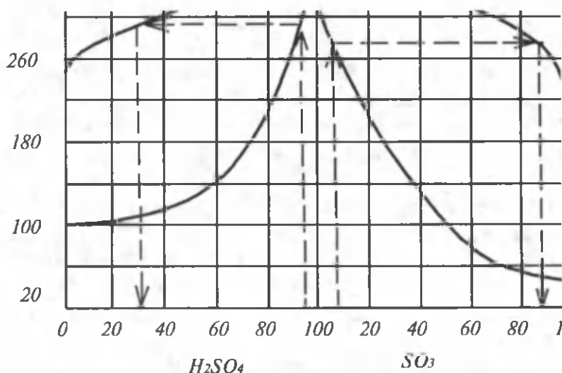
56- rasm. Atmosfera bosimida \text{H}_2\text{O}-\text{SO}_3 sistemasining qaynash diagrammasi.
