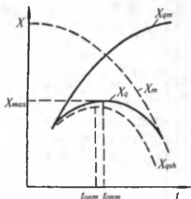
21- rasm. Ekzotermik jarayonlar uchun mahsulot unumining haroratga bog'liqligi. ( \tau, p, C_{ab}, S_{vb} = \text{const} ).
