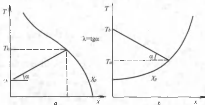
24- rasm. Ideal siqib chiqarish adiabatik reaktorlarida(mahsulotga) aylanish darajasining ortishi bilan haroratning o'zgarishi: a — ekzotermik, b — endotermik jarayon.
