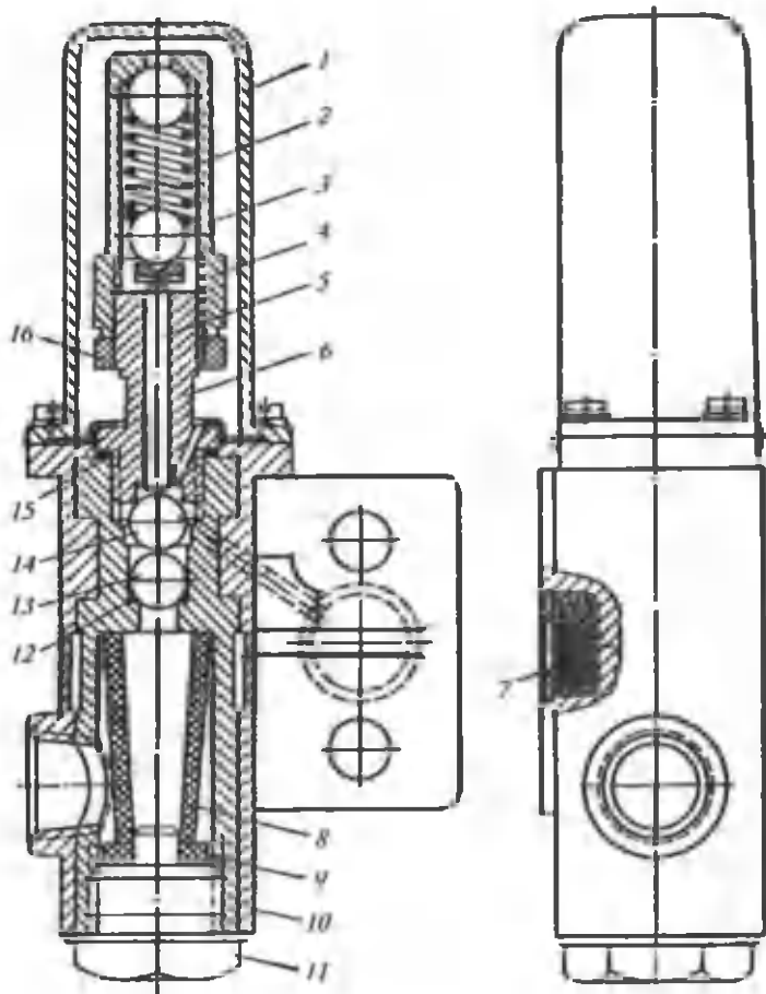
108-rasm. Bosim rostlagichi:
