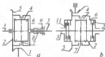
62-rasm. Differensiallar sxemasi:
