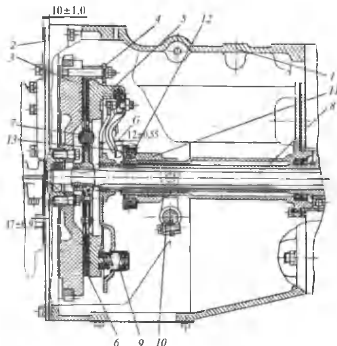
7-rasm. TTZ-100 traktorining ilashish muftasi:
