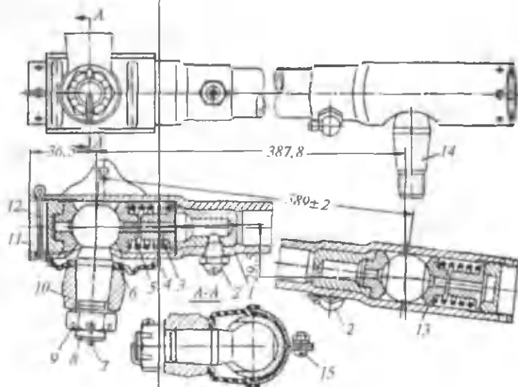
19-rasm. Bo'ylama rul tortqisi:
