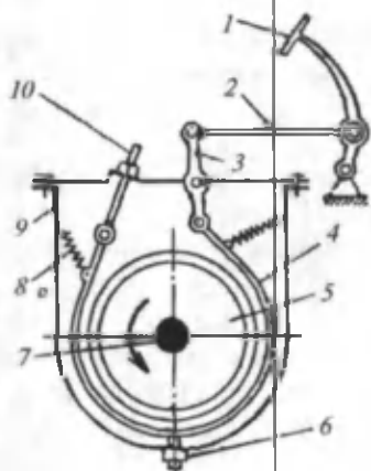
94-rasm. Tasmali baraban tipidagi tormoz sxemasi:
