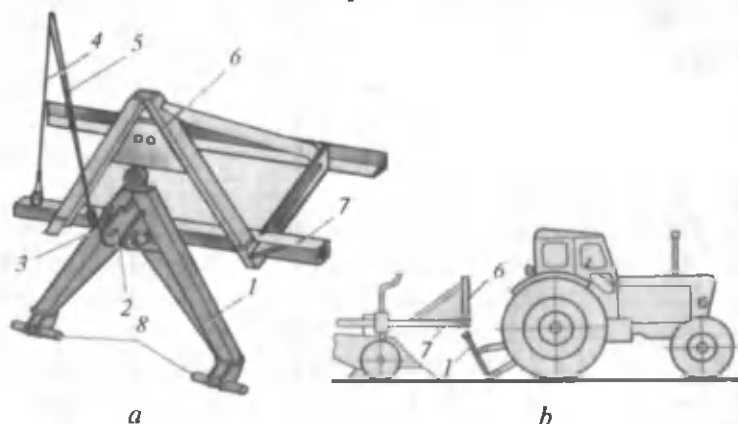
124-rasm. Avtotirkagich:
