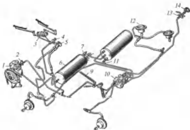
106-rasm. ЗИЛ-130 avtomobilining pnevmatik yuritmal tormoz tizimi jihozlarining sxemasi:
