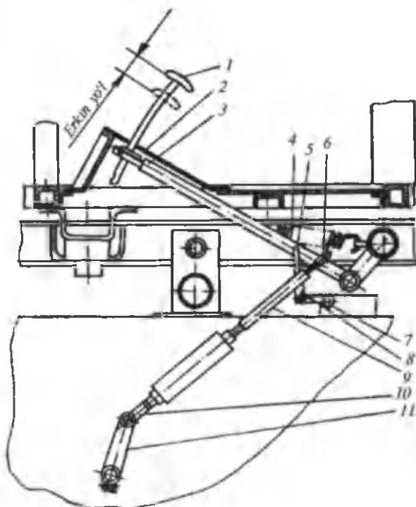
18-rasm. TTZ-100K11 traktorining ilashish muftasini boshqarish. 1- ilashish mufta pedali yostiqchasi; 2- kabina tagligi (polik); 3- ilashish muftasi pedali; 4- prujina; 5- blokirovka qurilmasining tortqisi; 6, 10- vilkalar; 7- blokirovka valigi; 8- blokirovka valigining richagi; 9- servomexanizm; 10- ajratish muftasini ajratish valigi. 11- tortqi.
