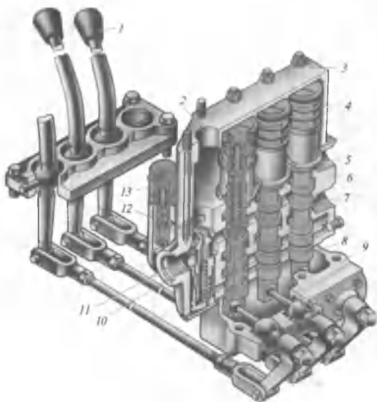
115-rasm. Hidrotaqsimlagich:
