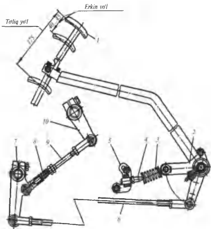
12-rasm. MT3-80 traktori ilashish muftasining mexanik yuritmasidagi prujinali kuchaytirgich:
