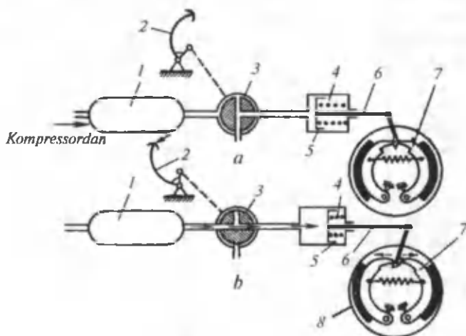
98-rasm. Pnevmatik yuritmalı tormoz tizimining soddalashtirilgan sxemasi: a — tormozlanmagan holat; b — tormoz ishlatilgan holat; 1- havo balloni; 2- tormoz pedali; 3- tormoz krani; 4- tormoz silindri; 5- porshen (diafragma); 6- shtok; 7- kolodkalar; 8- tormoz barabanini keruvchi moslama.
