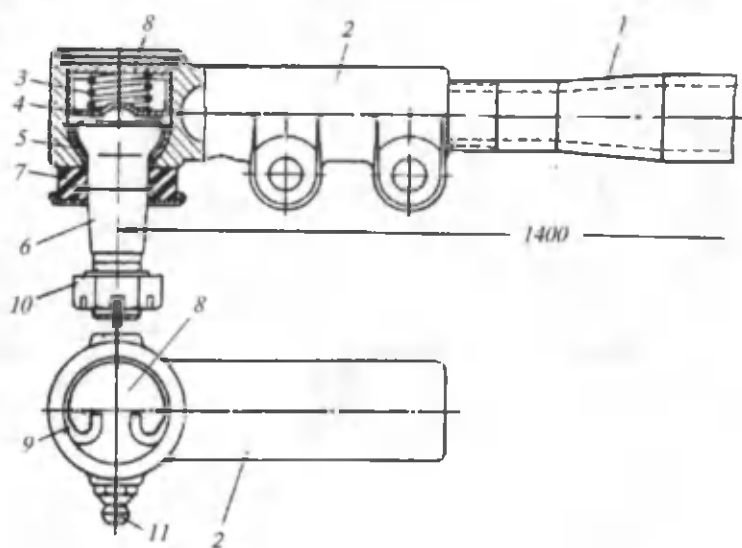
90-rasm. GA3-53A avtomobilining ko'ndalang rul tortqisi:
