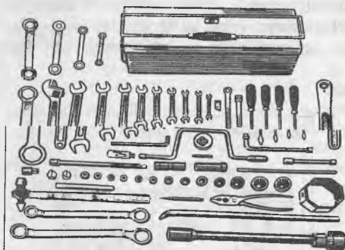
18-rasm. Avtochilangarning K-4670 rusumdagi metal idishli asboblari to'plami
