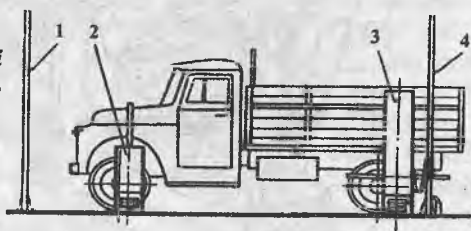
24-rasm. M129 modeli yuk avtomobillarini zarrachali yuvish jihozi
