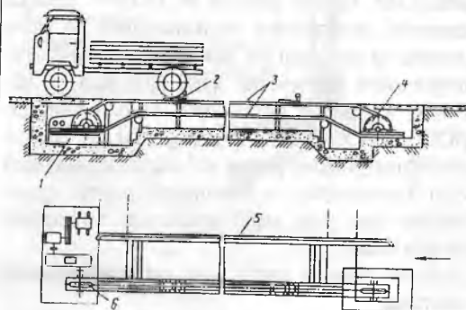
15-rasm. Iltirib yuruvchi konveyerning prinsipial shakli:
