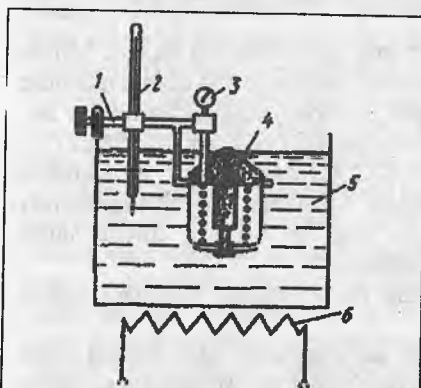
2.25-rasm. Termostatni tekshirish chizmasi
