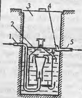
28-rasm. Moybenzintutgich
