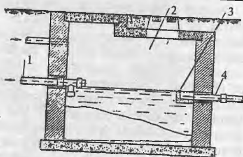
27-rasm. Loytingirich
