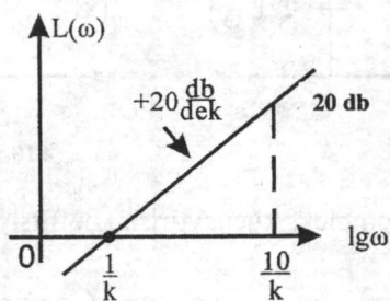
4.13-rasm. Differensiallovchi zveno uchun LACHX.
