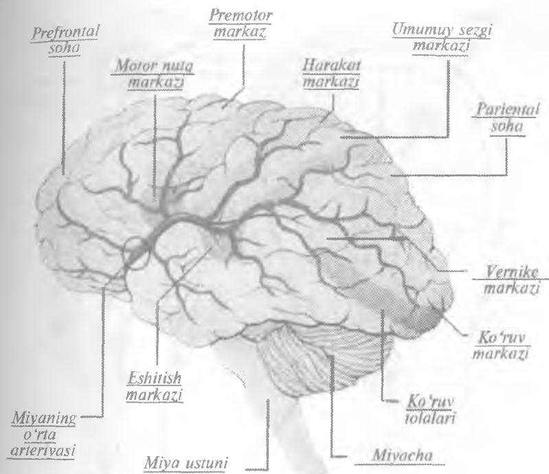
36-rasm. Bosh miya chap yarum shari.
