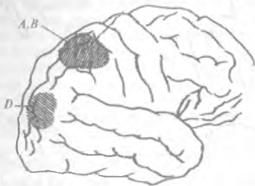
7-rasm. Bosh miya o'ng yarim sharining tepa va ensa sohalari
