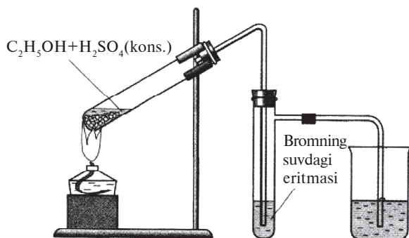
6- rasm. Etilenning laboratoriyada olinishi.
