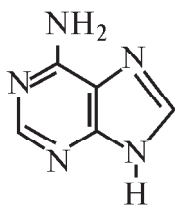
adenin (a)
