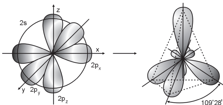
1- rasm. Uglерod atomining sp^3 - gibrldlanishi.
