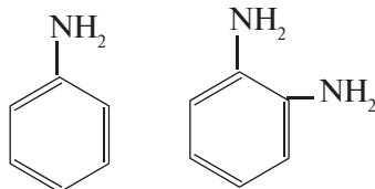
monoamin
