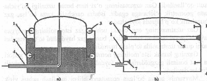
9.2-rasm. Past bosimli gazgolderlarning prinsipial sxemasi: a- ho'li;
