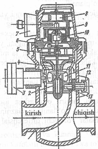
4.9-rasm. TOR-1 suyuqlik sarf o'lchagich.
