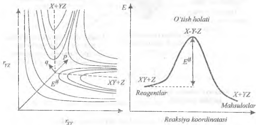
32-rasm. XY+Z \rightarrow X+YZ reaksiyaning sirt potensial energiyasi: nuqtali chiziq — reaksiya koordinatasi q , streika — q ning yo'nalishi va E^\# nuqtada uning orthogonal koordinatalari p .
