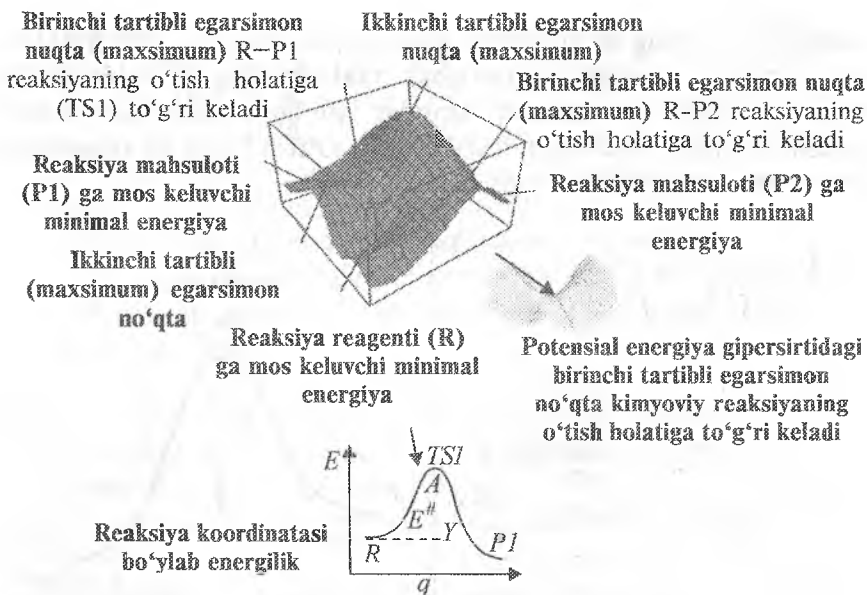
34-rasm. Sirt potensial energiyasining modeli.
