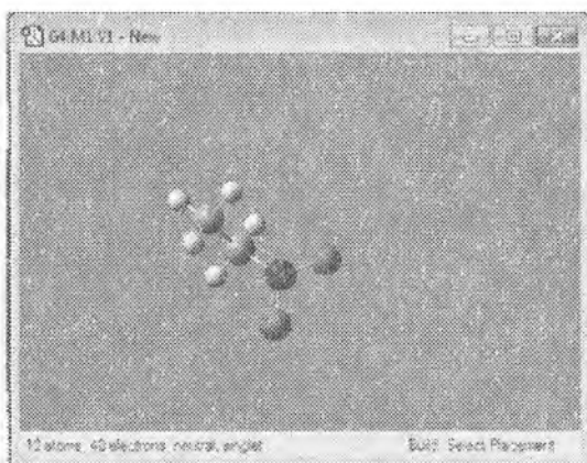
9-rasm. Nitroctan molekulasini.
