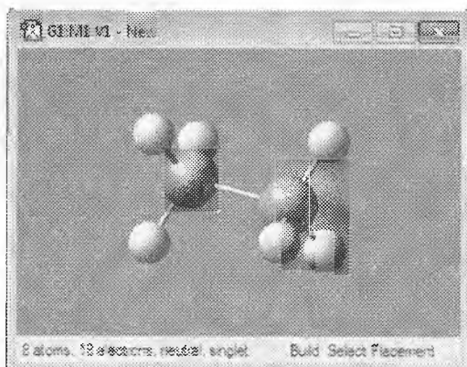
5-rasm. Etan molekulasini yasash.
