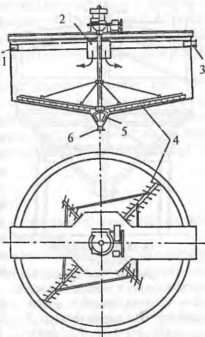
11-rasm. Suspenziyani markazdan uzatadigan tipaviy tindirgich:
