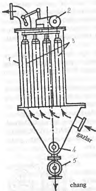
41-rasm. Yeng suzgich: 1 — qobiq; 2 — silkitib qoqish; 3 — yenglar; 4 — shnek; 5 — yopqich (lo'kidon).
