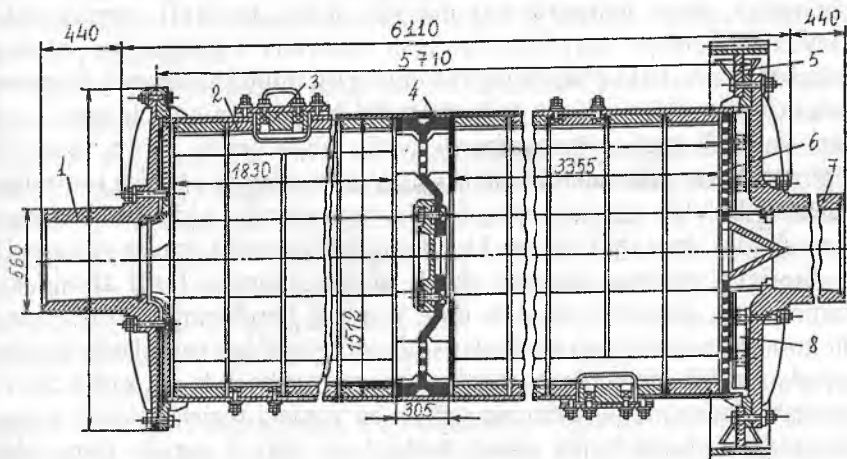
21-rasm. Barabanli ikki bo'lmali tegirmon: 1,7 — sapfalar; 2 — himoya plitasi; 3 — lyuk; 4 — diafragma; 5 — shesterna; 6 — bo'shatish panjarasi; 8 — liftiyorlar.
