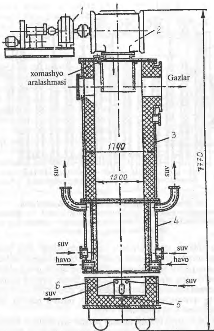
35-rasm. Natriy sulfid olish uchun shaxtali pech:
