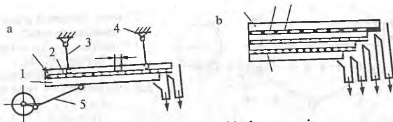
26-rasm. Elakli g'alvir mashinalar sxemasi:
