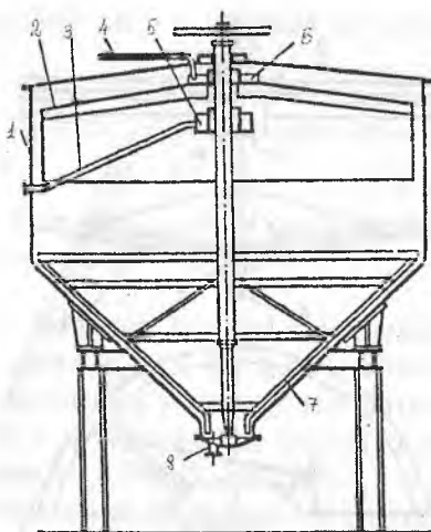
12-rasm. Tindirgich-dekanter:
