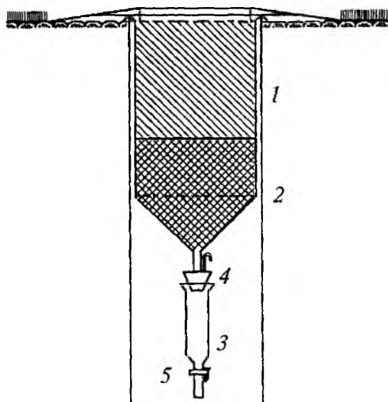
17-rasm. A.V.Klyucharev kichik hajmli metall lizimetrlining kesmasi.
